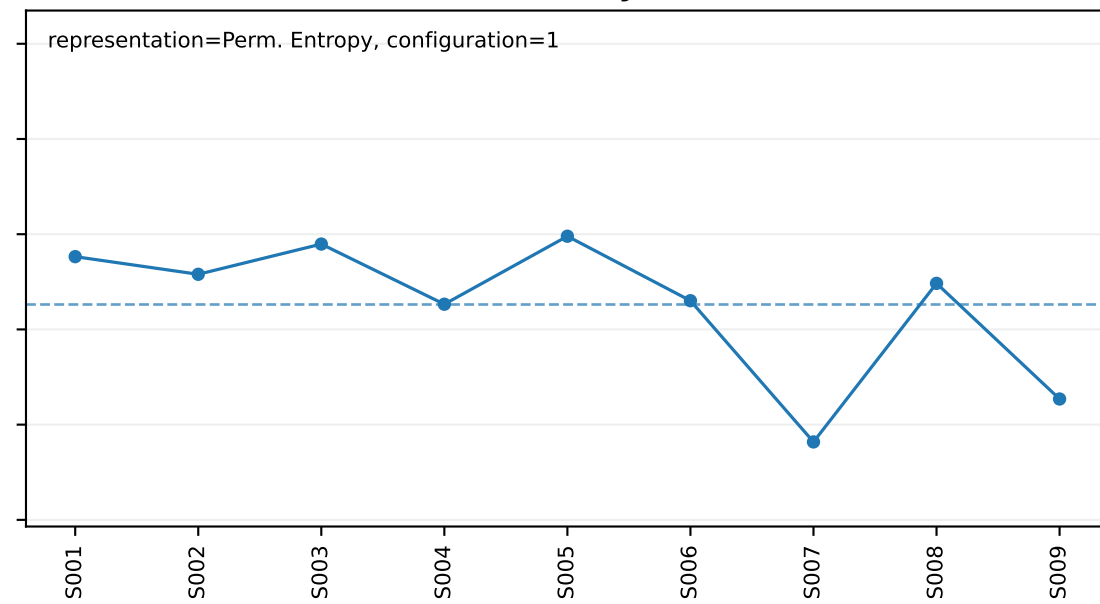
Cross-subject
