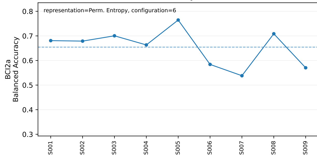
Intra-subject
