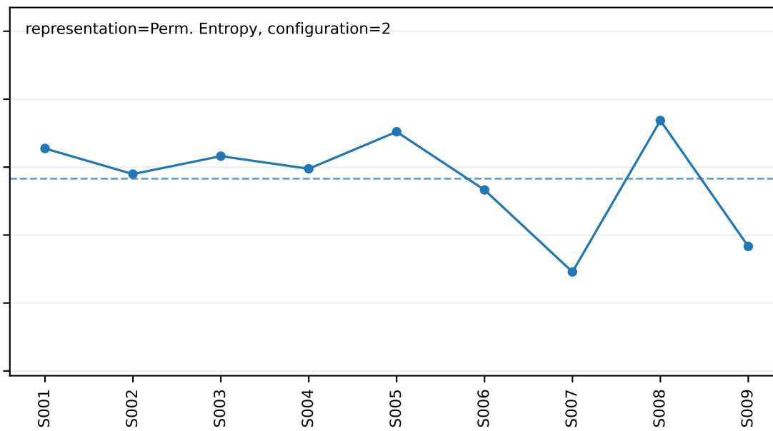
Cross-session
